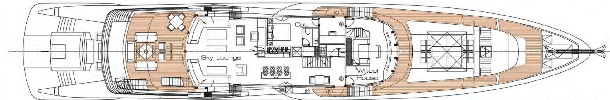
Bridge Deck
